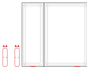
Floor stabilizing foot 1ML0120 L 15 \frac{3}{4} P 3 \frac{3}{4} H 1 \frac{1}{4}
