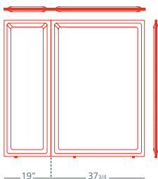
Acoustic panel H 55" 1ML0140 L 56 \frac{3}{4} " P 1 \frac{3}{4} " H 15 \frac{3}{4} "
